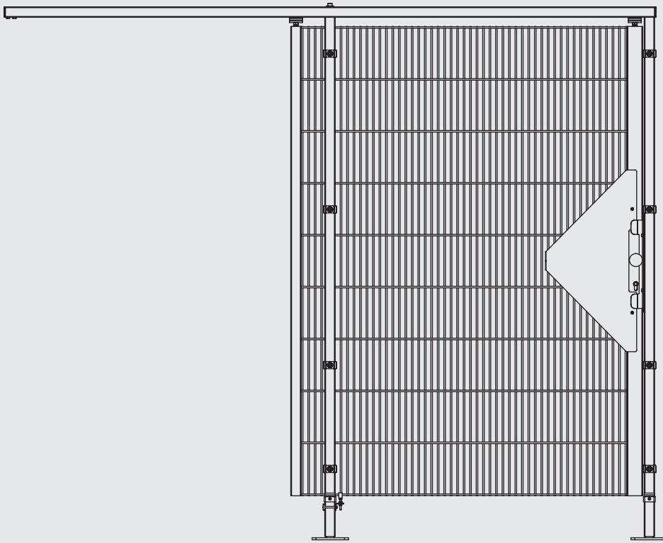
1-leaf Sliding door, variant TS01, installation (page 10-35)
